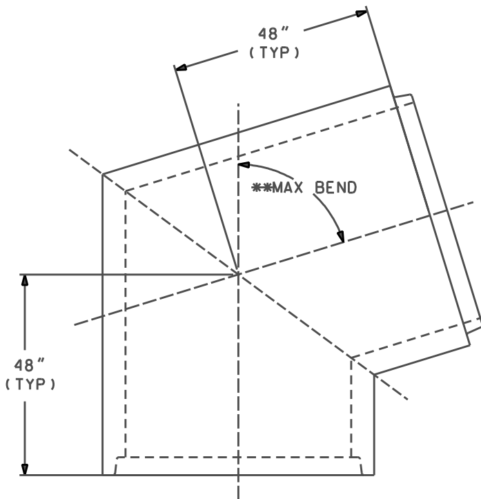
SINGLE SECTION BEND (TYP)
