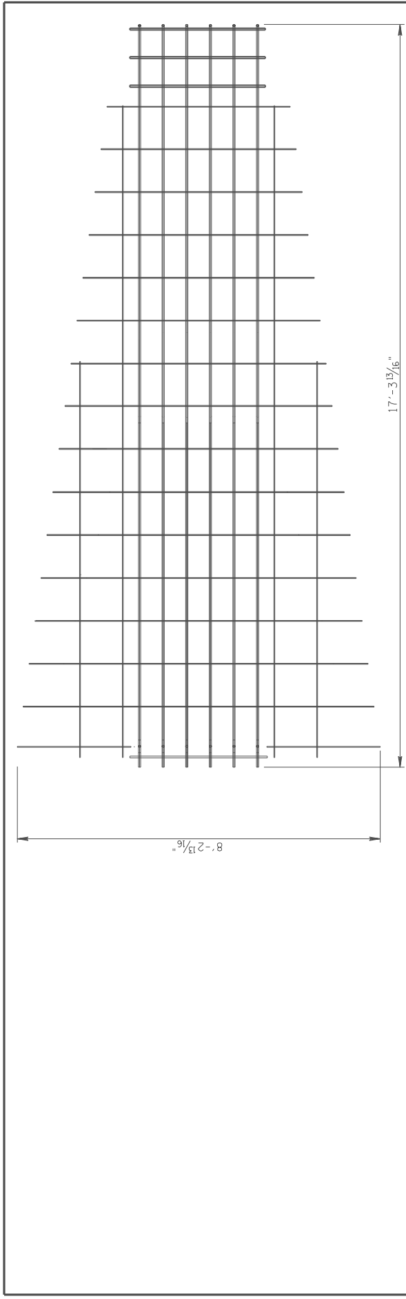
COMBINED MAT 1 AND MAT 2 (SHOWN WITHOUT BENDS)
