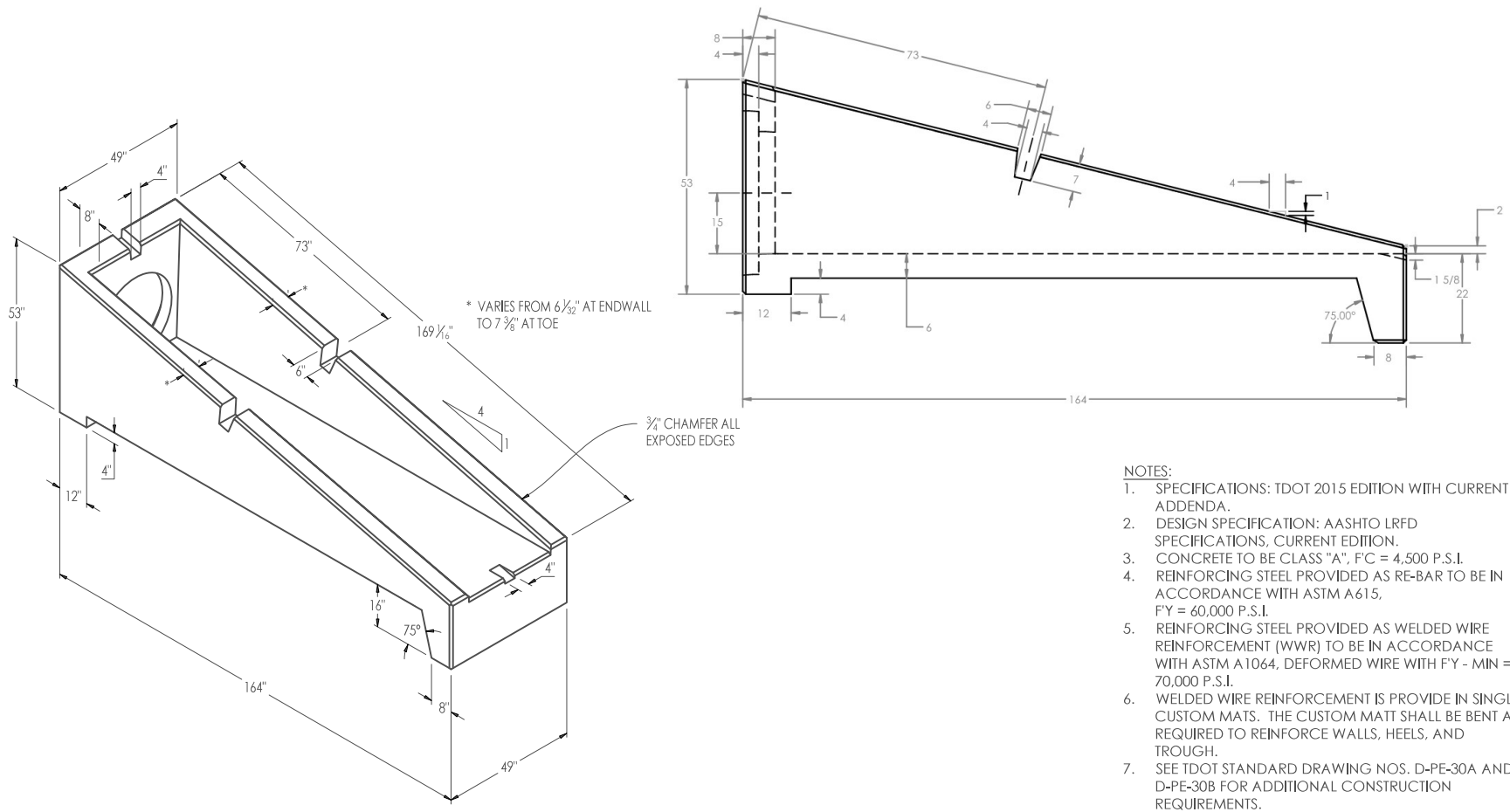
ISOMETRIC VIEW SHOWING DIMENSIONS, 4:1 SLOPE
