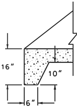
TOE DETAIL
