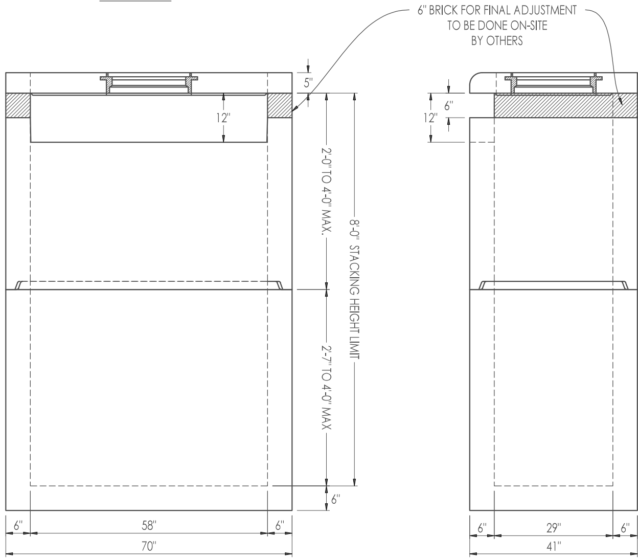
FRONT ELEVATION
