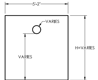
4" BAFFLE WALL Scale 1/4"=1'-0"
