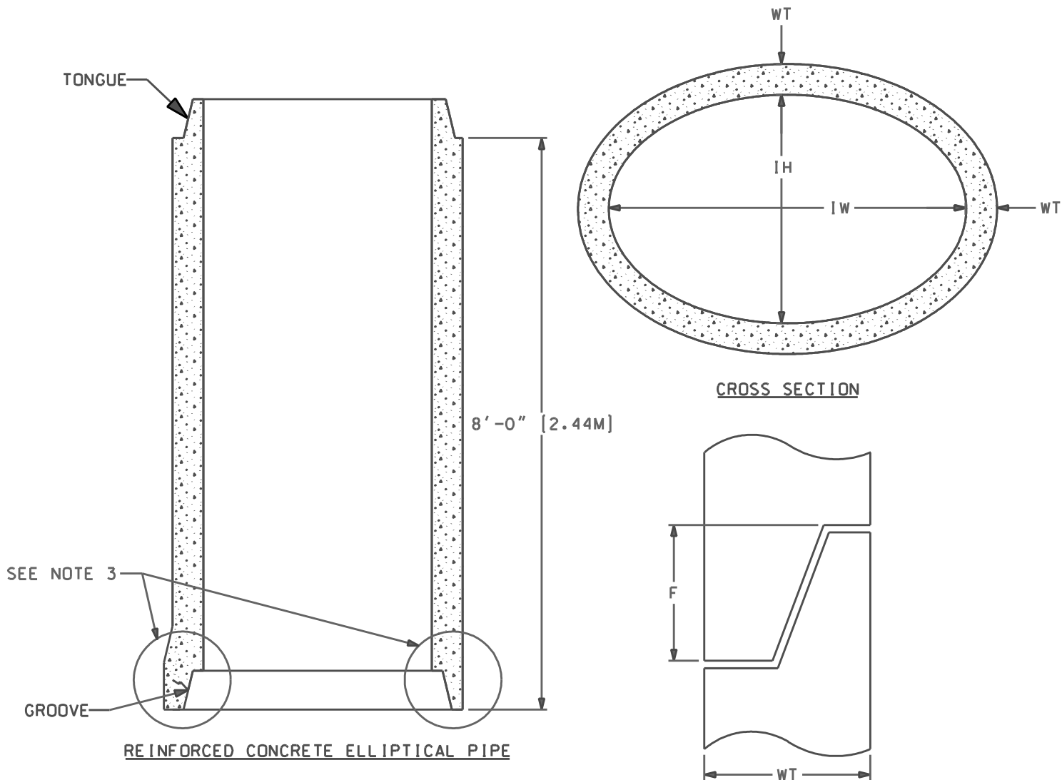
JOINT DETAIL
