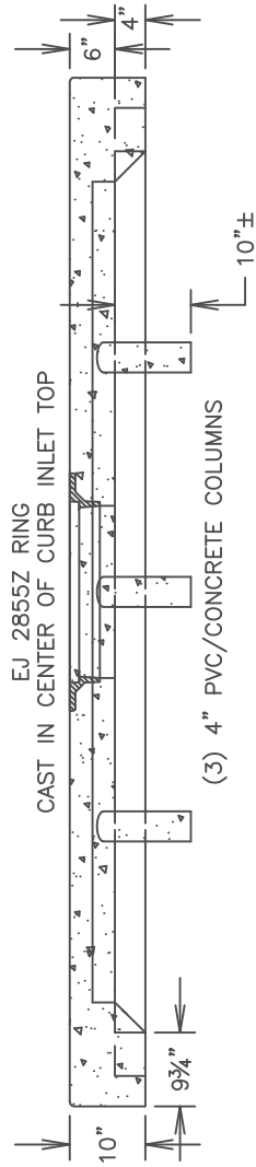
FRONT VIEW
