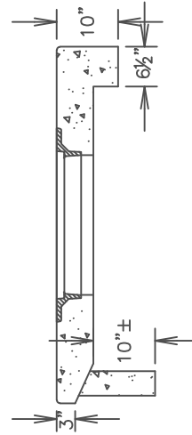
SIDE SECTION VIEW
