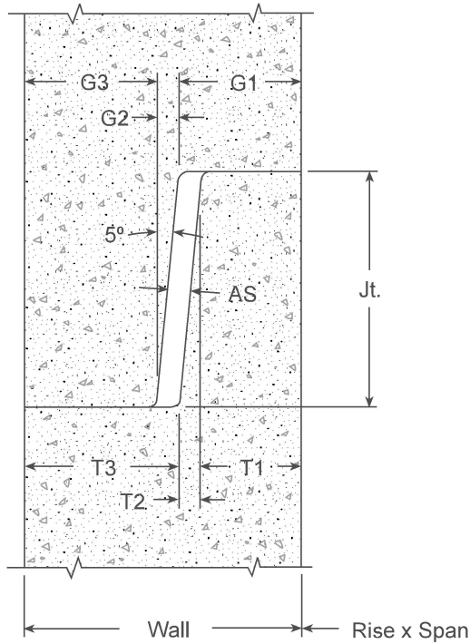
Joint Detail
