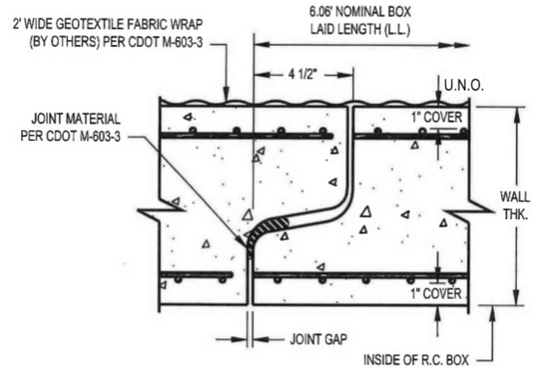
TYPICAL SECTION THRU BOX JOINT
