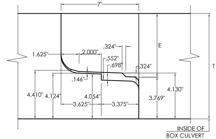
TYPICAL SECTION THRU BOX JOINT
