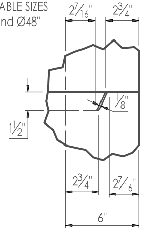
JOINT DETAIL
