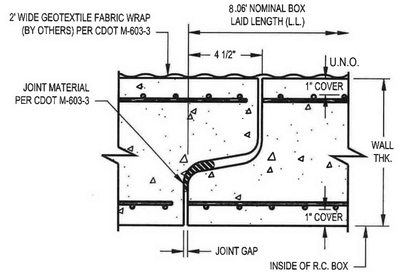
TYPICAL SECTION THRU BOX JOINT
