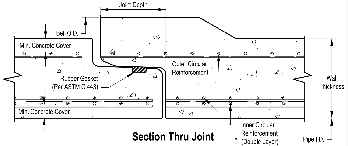
36"Ø to 72"Ø RCP (Big Bell Confined 'O'-Ring Joint) w/ Double Inner & Outer Cage Reinforcement
