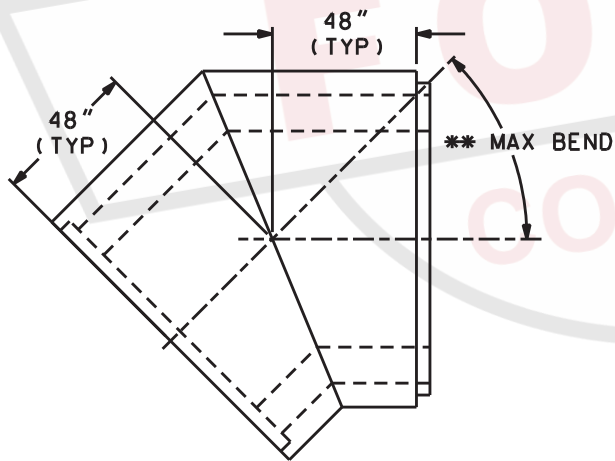
SINGLE SECTION BEND (TYP)
