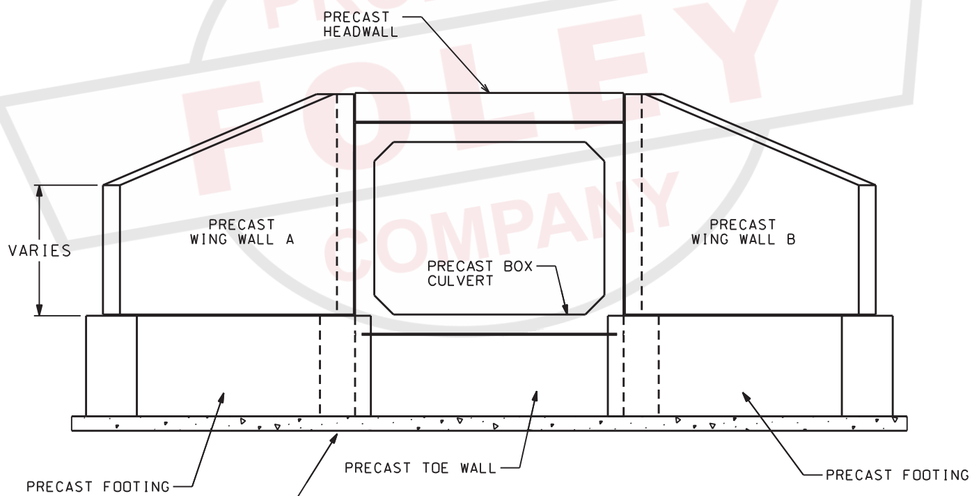
ELEVATION VIEW
