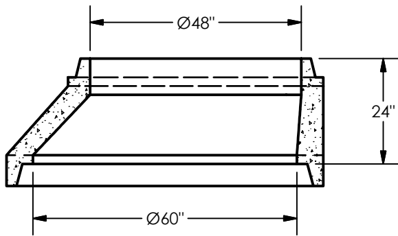
Ø5' TO Ø4' CONICAL REDUCER 1.15 TONS
