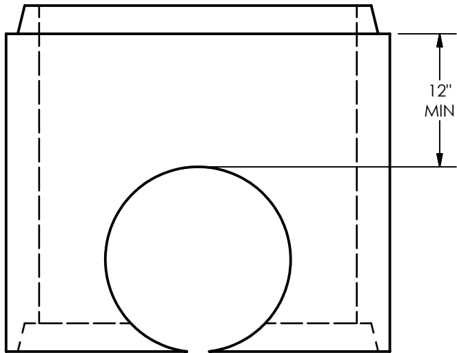
CORED DOGHOUSE RISER (TYPICAL)
