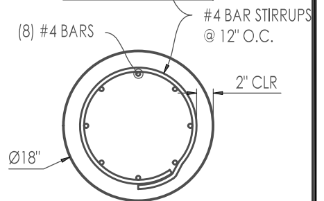
PLAN & ELEVATION
