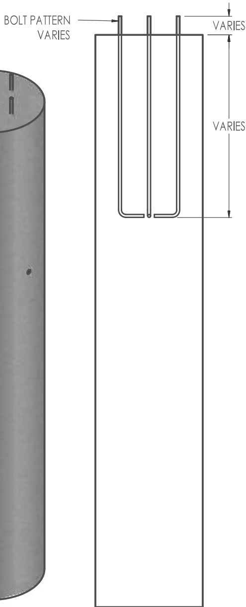
ANCHOR BOLT DETAIL
